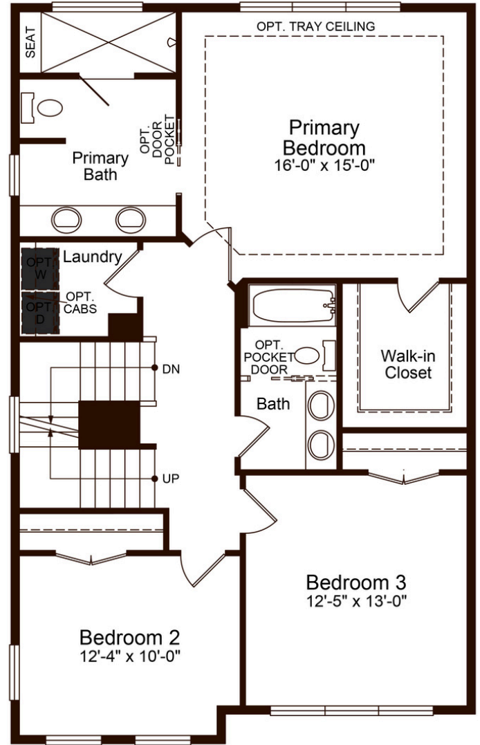
SECOND FLOOR W/ LOFT
