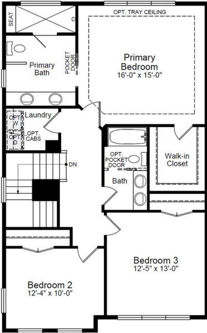
STANDARD SECOND FLOOR
