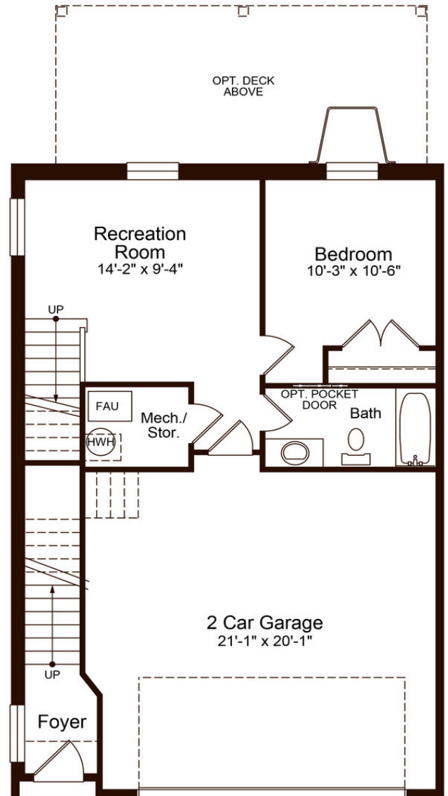
OPTIONAL LOWER LEVEL W/ BEDROOM AND FULL BATH
