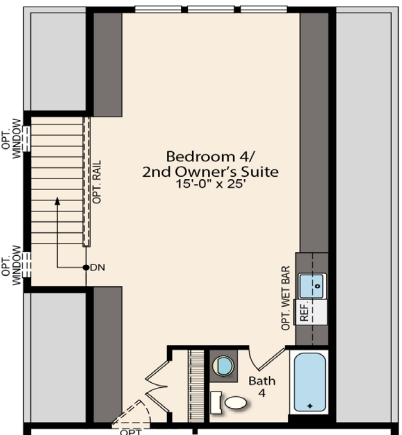
Opt. Extended 2nd Fl. Suite (Shown w/ Opt. Rear Garage Stairs
