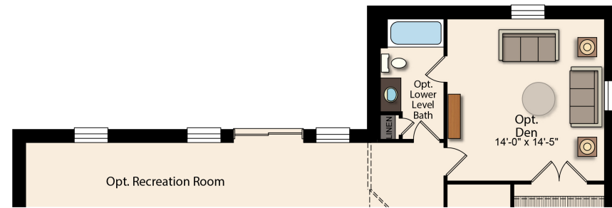
Opt. Finished Lower Level Partial Plan W/ Opt. Walkout
